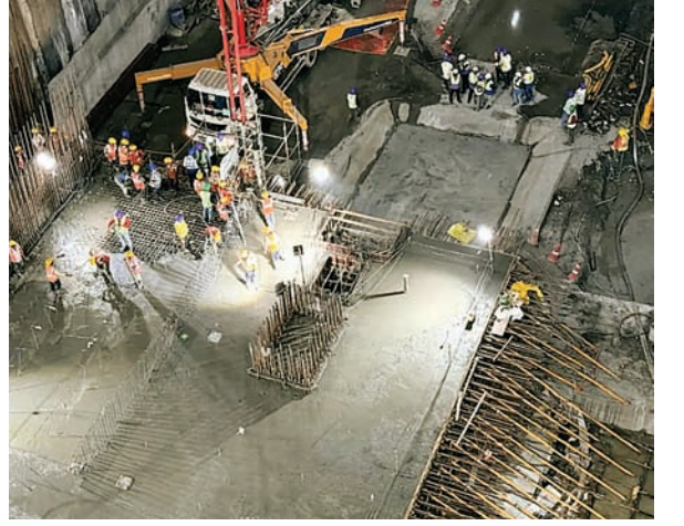
69 slabs that are cast for the station, which will form the deepest construction level for the Bullet Train station.
